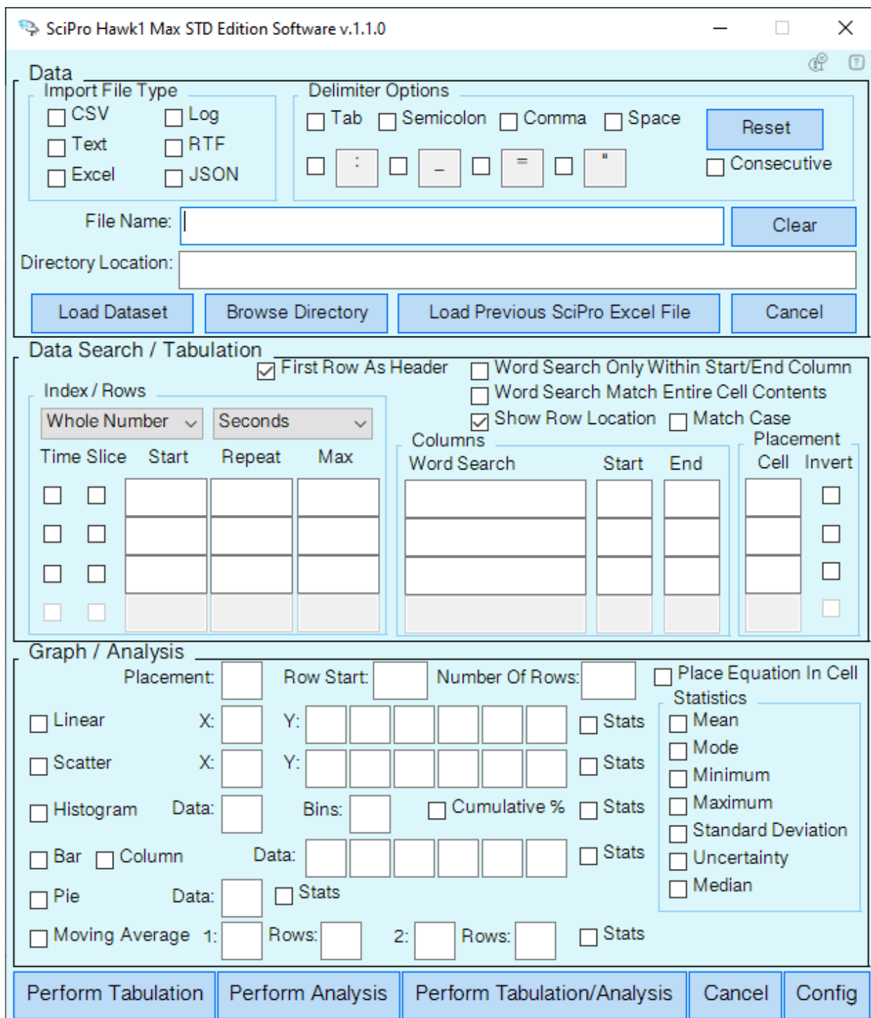
Figure 7: SciPro Hawk1 GUI
