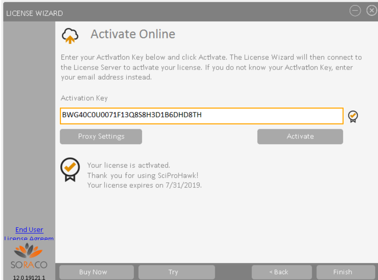
Figure 6: Activate online
