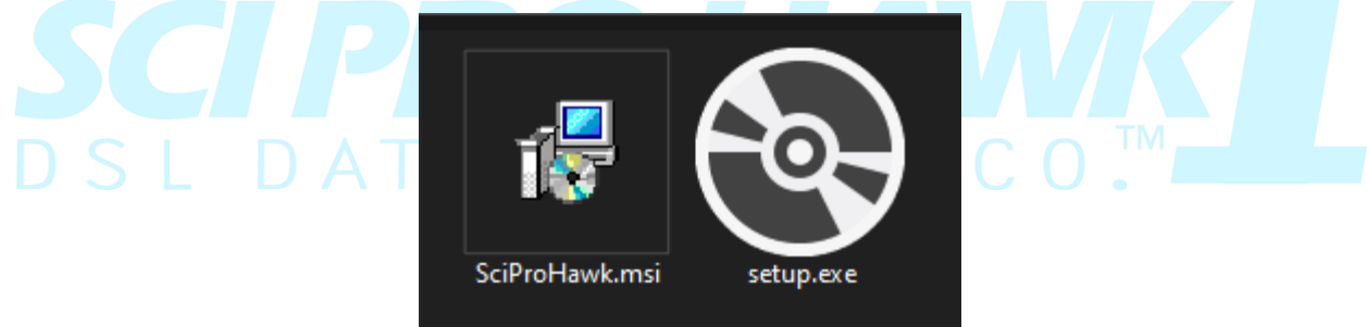
Figure 1 : Installer
