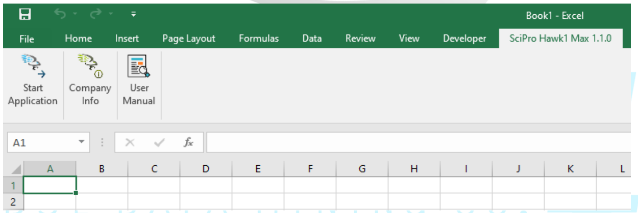
Figure 3 : SciPro Hawk1
