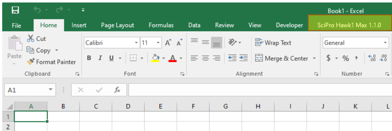
Figure 2: Excel Ribbon
